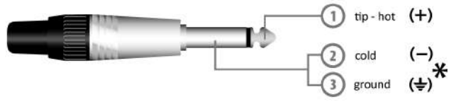
LINE IN, various OUT Jack (unbalanced)
