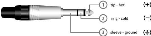
LINE IN, various OUT Jack (balanced)
