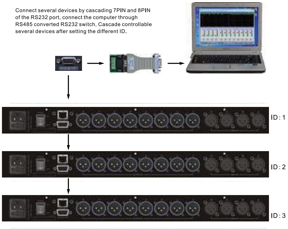
The 7PIN is: RS485 D+ , 8PIN is: Rs485 D- of the RS232 port.
